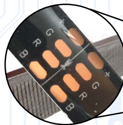
Cut Between Copper Plates Locations marked with Scissor icon
